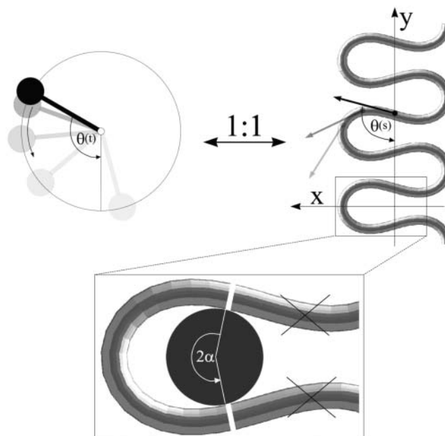
FIGURE 2 The Kirchhoff kinetic analogy between the spinning top and the bent/twisted rod depicted for a special case: the plane pendulum–planar rod equivalence. The inset shows how an intranucleosomal loop can be constructed by inscribing the octamer (gray disk) into the bent rod. The nucleosome opening angle 2\alpha accounts for the adsorption energy cost (see text for details).
