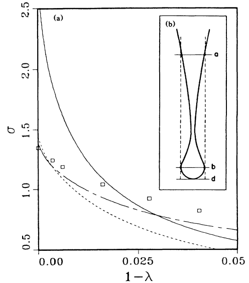
FIG. 2. (a) Variation of \sigma with 1 - \lambda . The solid line gives p = 1 , v = 2 , and k = 0.1 . The chain-dashed line gives p = 0.01 , v = 2 , k = 0.95 , and is essentially identical to that given by the method of DH, where k = 1 and p \rightarrow 0 . Data points represent a numerical solution of the Saffman-Taylor equations by McLean (Ref. 14), to which the DH method should also apply. The dashed line gives p = 0.01 , v = 2 , and k = 0.1 . (b) Schematic drawing of the lower part of a groove with a bubble closure.
