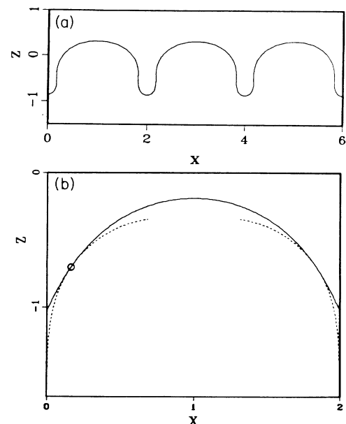
FIG. 1. (a) Finite-amplitude solution of Eq. (8) for p=3 , v=2 , k=0.1 , and \sigma=0.29 with B chosen to satisfy conservation condition (5). (b) The (outer) solution of Eq. (8) for p=1 , v=2 , k=0.1 , \sigma=0.78 , and 1-\lambda=0.03 (solid line), and an associated inner solution of Eq. (9) (dashed line), determined approximately by “patching” the function and its derivative to the outer solution at the point indicated. As \lambda \rightarrow 1 , this is essentially equivalent to the asymptotic matching procedure of DH.
